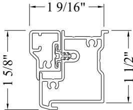
Base w/2" Brickmould Snap Cover
